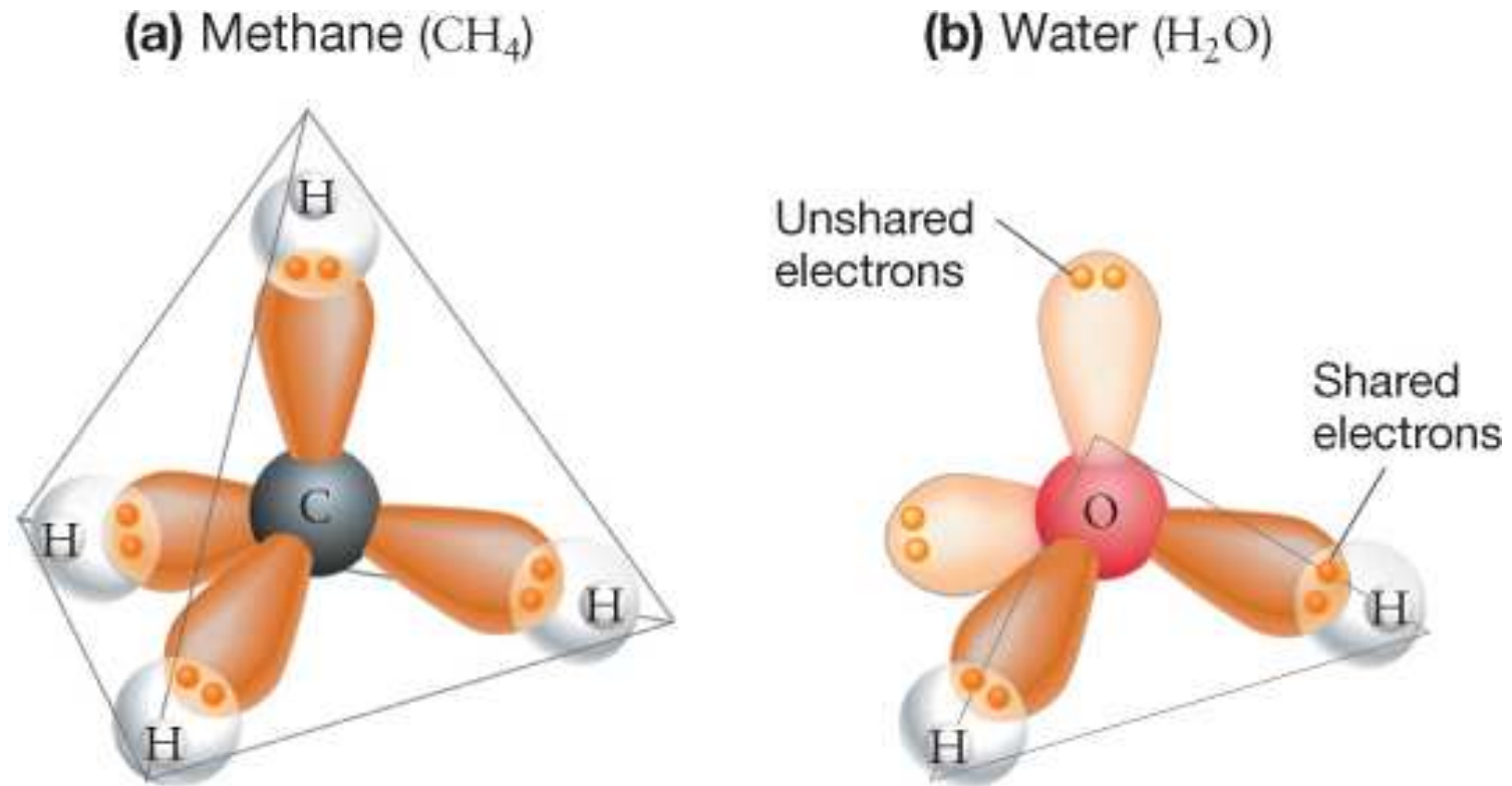
Figure 2.9 The Geometry of Methane and Water.
