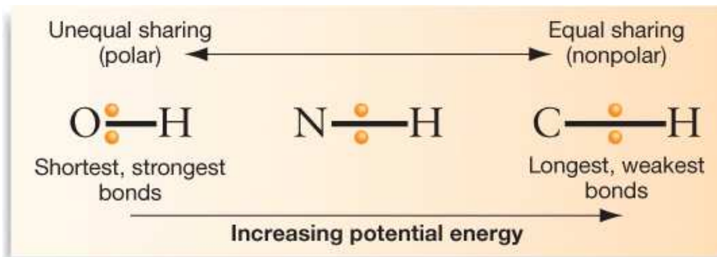
Figure 2.17 Potential Energy as a Function of Electron Sharing.
