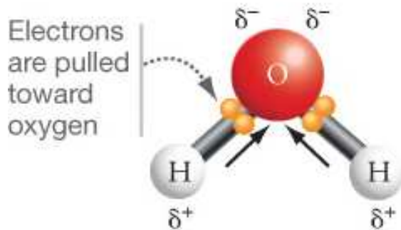
(a) Water is polar.
